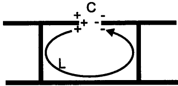
Figure 3 Origin of the capacitance and inductance in the effective medium model.
