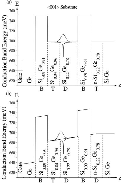
FIG. 7. The band structure diagram for the spin-resonance transistor, with epilayers grown in the \langle 001 \rangle direction. Both the unbiased (a) and the biased case (b) are shown. The conduction band energies allow the selection of layers with composition D, T, and B such that the confining barrier height is increased to 50 meV, while the strain in the layers is reduced, compared to the \langle 111 \rangle orientation. The epi-layer thicknesses are not to scale.
