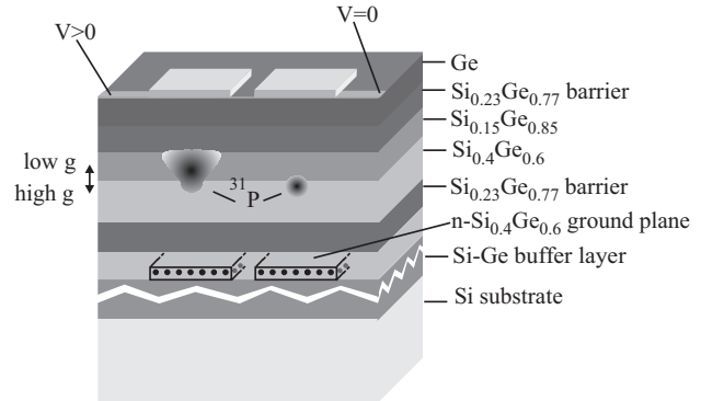
FIG. 5. The left transistor gate is biased V > 0 producing single qubit unitary transformations in the left SRT. The right gate is unbiased, V = 0 . The n\text{-Si}_{0.4}\text{Ge}_{0.6} ground plane is counter-electrode to the gate, and it also acts as an FET channel for sensing the spin.
