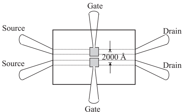
FIG. 11. Top view of the proposed device to demonstrate a CNOT gate. A perspective view (, not including the source and drain,) is shown in Figure 5. Fluctuations in the current that flows from source to drain signal the charge state of the dopant ion under each electrode.
