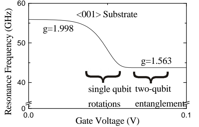
FIG. 8. A schematic of the dependence of the spin resonance frequency on the transistor gate voltage for the case of a \langle 001 \rangle substrate. The static magnetic field is in the \langle 001 \rangle direction and has a strength of 2 Tesla. The tuning range is reduced in this growth direction with respect to the \langle 111 \rangle case, because the g -factor in the Ge-rich layer is different: g = 1.563 .
