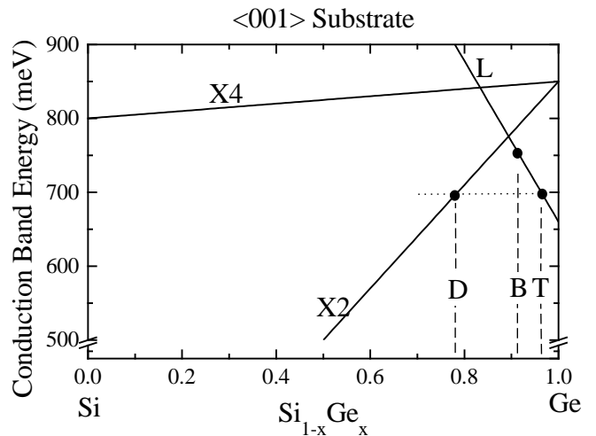
FIG. 6. The conduction band energy in Si-Ge alloys, compositionally strained in the \langle 001 \rangle direction, from neutral strain at 100% Ge. The L-valley has 4 minima that remain degenerate. The X-valley has 6 minima along the cubic directions, that are split between X4 and X2. The compositions D, T, and B are much less strained than in the \langle 111 \rangle case, and allow for higher barrier heights to confine the dopant electron. For this crystal orientation, the g -factor in the Ge-rich T- and B-layers is g = 1.563
