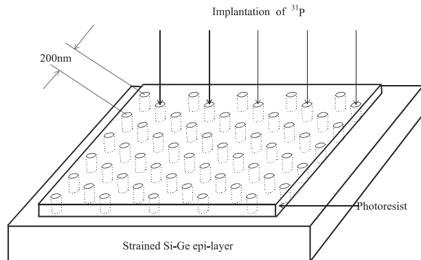
FIG. 12. The ion implantation step for inserting an array of qubit donor ions. The buried FET channels, that act as counter-electrodes to the gates and sense the spin/charge state, would be produced the same way. In a small-scale demonstration, the array would consist of only 2 rows, aligned with the FET channels of Figure 11. This should provide an adequate yield of good qubit pairs.
