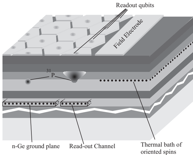
FIG. 15. A perspective view of Figure 14, gives more details of the readout architecture for the peripheral qubits. The field electrode allows the Readout Qubits to interact with the heat bath of oriented electron spins
