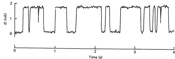
FIG. 10. The current noise in a small FET at 83 K from Kurten et al [37]. At this temperature the channel current fluctuates between two states, caused by a single trap being filled and emptied by a single charge. The change in channel current is \approx 2 nAmps, which represents a few percent of total channel current, and is easily measured.
