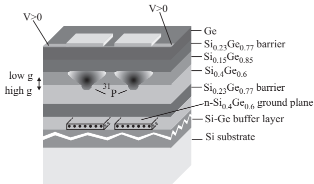
FIG. 9. Attracting the electrons to the \text{Si}_{0.23}\text{Ge}_{0.77} B-barrier reduces their Coulomb binding energy and increases their wave function overlap, allowing 2-qubit interaction.
