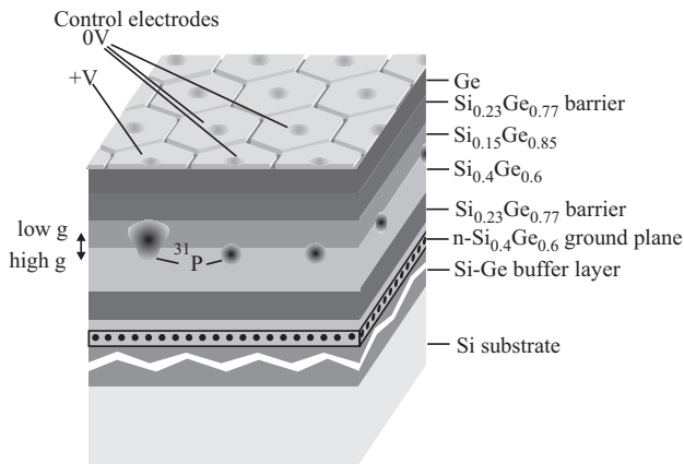
FIG. 13. In the future, we can expect arrays of Si-Ge SRT transistors. The center-to-center spacing would be \approx 2000 Å. The gate electrodes on top will perform both single and 2-qubit operations, and can be used for data and instruction read-in.
