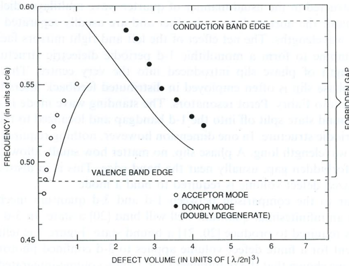
Figure 7 Donor and acceptor mode frequencies as a function of normalized donor and acceptor defect volume. The points are experimental and the corresponding lines are calculated. Defect volume is normalized to [\lambda/2n]^3 where \lambda is the mid-gap vacuum wavelength and n is the refractive index. A finite defect volume is required to bind a mode in the forbidden gap.
