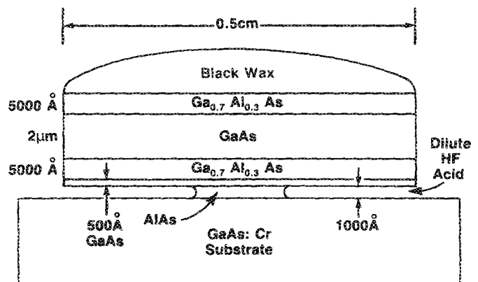
FIG. 1. Macroscopic epitaxial films can be undercut by dilute hydrofluoric acid. The AlAs release layer is shown as 1000 Å thick but has been as thin as 20 Å. In actual practice, the tension in the wax supporting layer lifts up the edges of the film as shown in Fig. 3.
